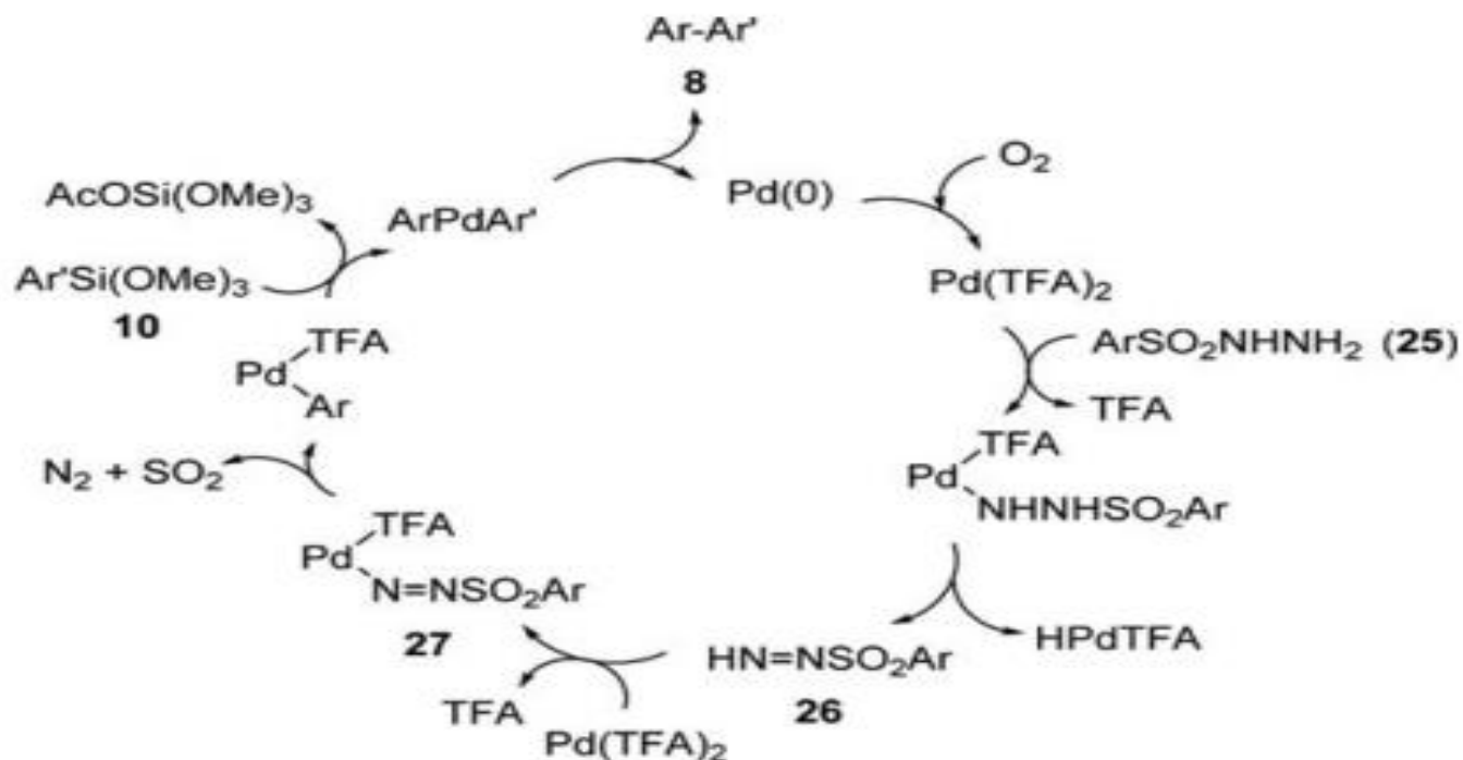
Scheme 15. Proposed mechanism for the coupling between hydrazines and the silane 10 .
