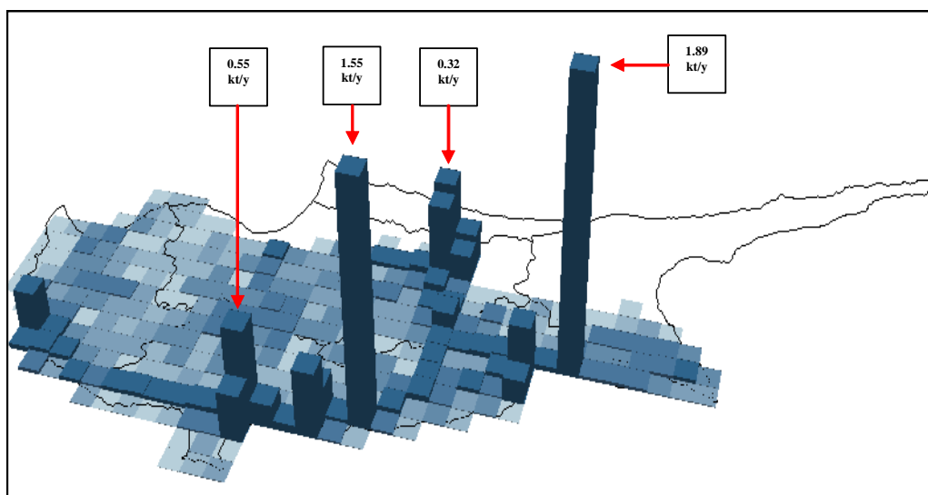
Figure 3. Spatial allocation and peak values of total NMVOC emissions
