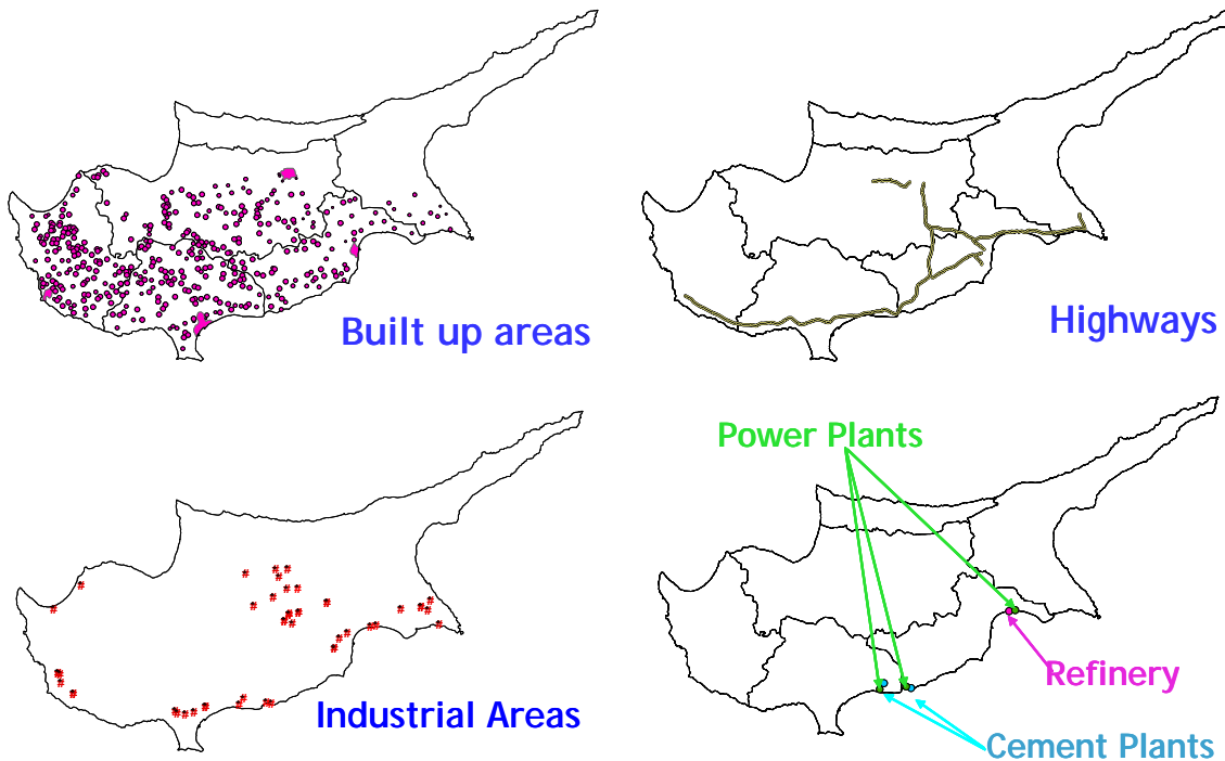
Figure 1. Spatial allocation of major emission sources
