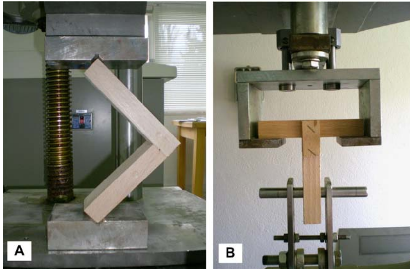
Figure 3. Loading in compression of the corner joint specimens (A), Loading in tension of the middle joint specimens (B)
