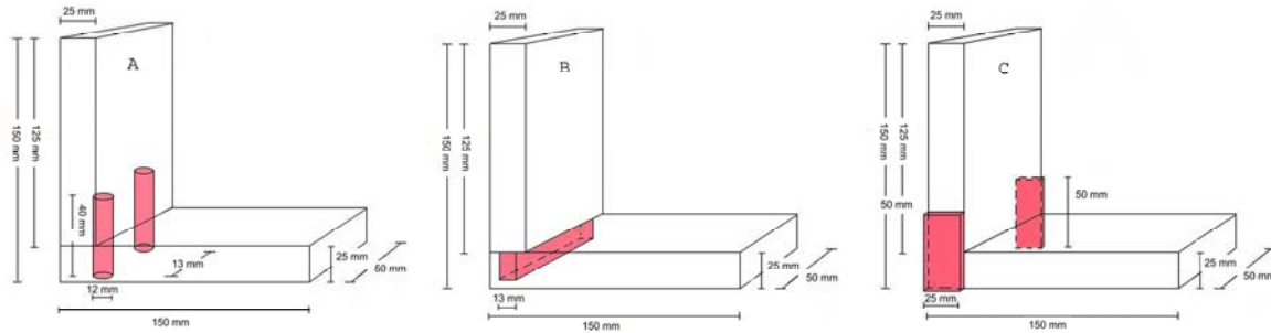
Figure 1. Dowel corner joint (A), Mortise - Tenon corner joint (B), Gusset Plates corner joint (C)
