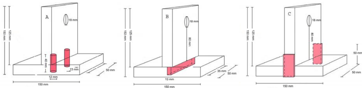
Figure 2. Dowel middle joint (A), Mortise - Tenon middle joint (B), Gusset Plates middle joint (C)
