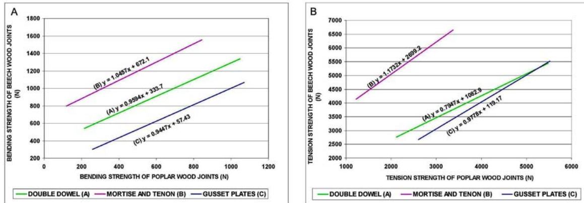
Figure 4. Equations of covariance between values of beech wood joints and values of poplar wood joints in bending (A) and tension (B) strength
