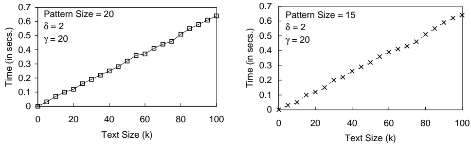
Fig. 4. Timing curves for the SHIFT-PLUS Algorithm.
