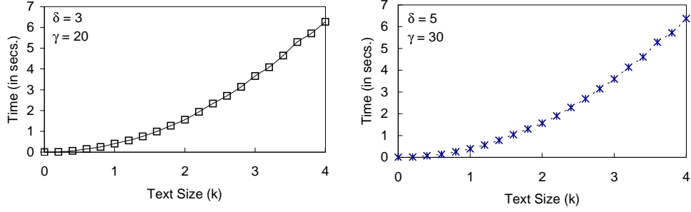
Fig. 7. Timing curves for \{\delta, \gamma\} -approximate squares.
